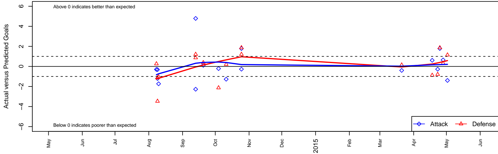
SSC Shadow United Dickson G03 Dots are actual minus expected GF (blue circles) and GA (red triangles). Blue line is smoothed change in attack strength. Red is smoothed change in defense strength.
